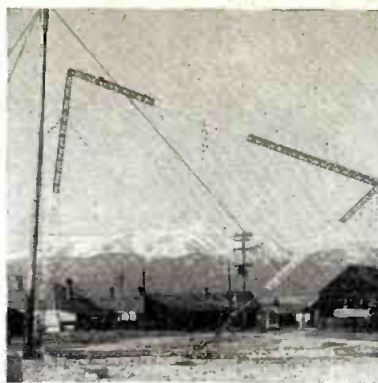
A SUDDEN gust of wind recently snapped off a tower being constructed for KLVV Leadville, Col. At the time it crashed, the tower had reached 160 feet. The crashed tower frames Mt. Massive, lofty peak of the Rockies
